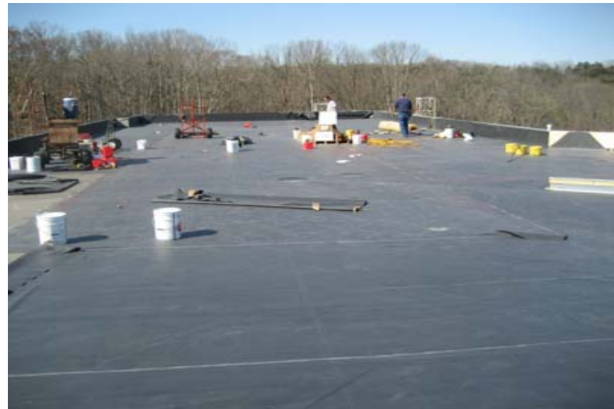
April 9, 2009 - The rubber roof membrane is being installed on the A1 building section
